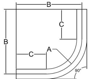
90° dimensional drawing
